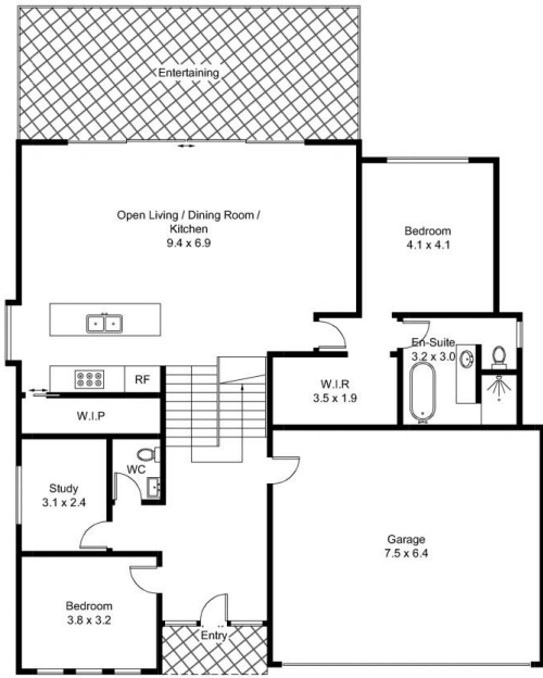
Ground Floor = 199.3 Sq M
